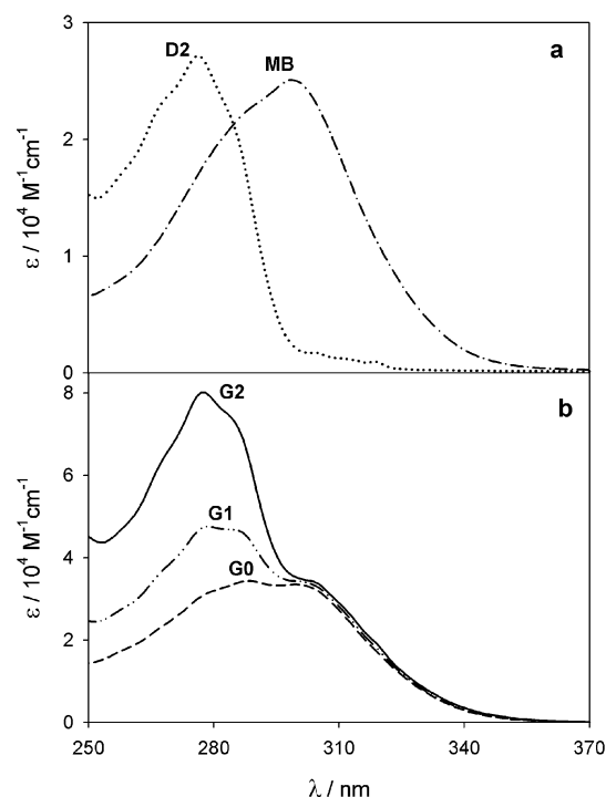
Fig. 1 Absorption spectra of MB and D2 (a) and dendrimers G0–G2 (b) in \text{CH}_2\text{Cl}_2\text{-CHCl}_3 1 : 1 (v/v) at 298 K.
